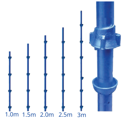
CUPLOCK STANDARDS
